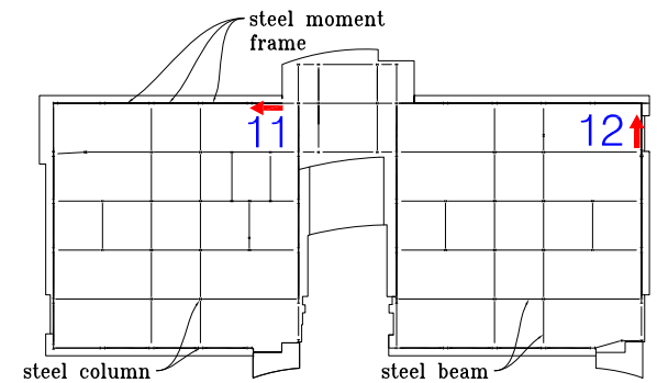
Level 4 Plan
