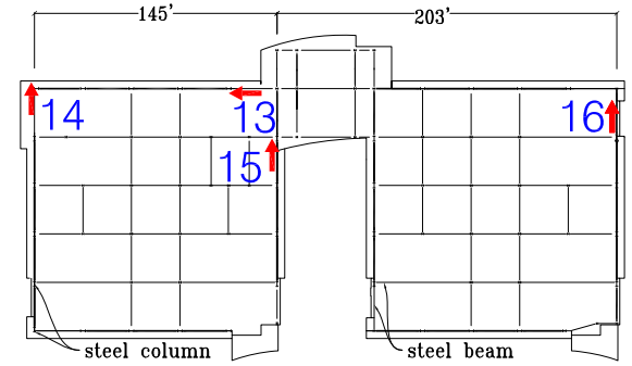
Roof Plan
