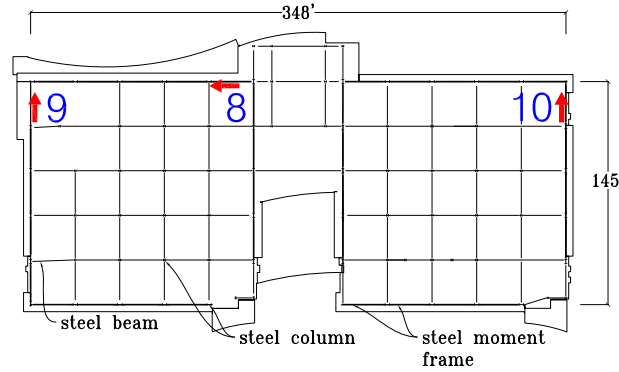
Level 3 Plan
