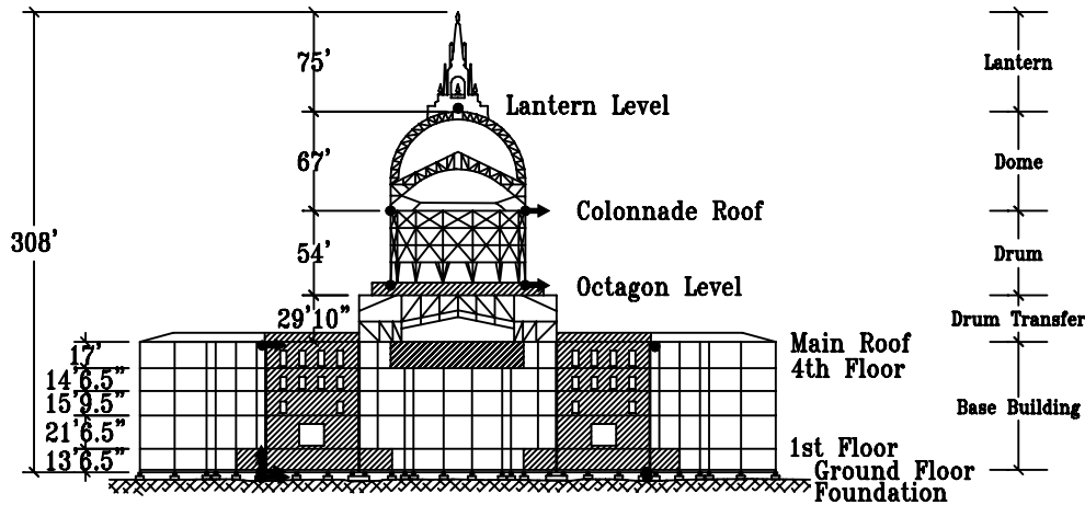
East Elevation
