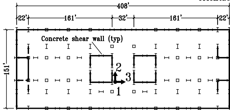
Basement Plan
