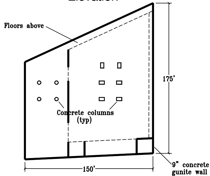
Foundation Plan
