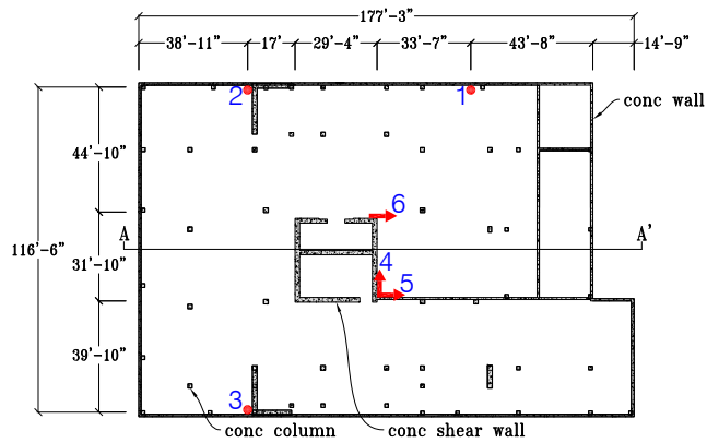
Lower Level 3/ Foundation Plan
