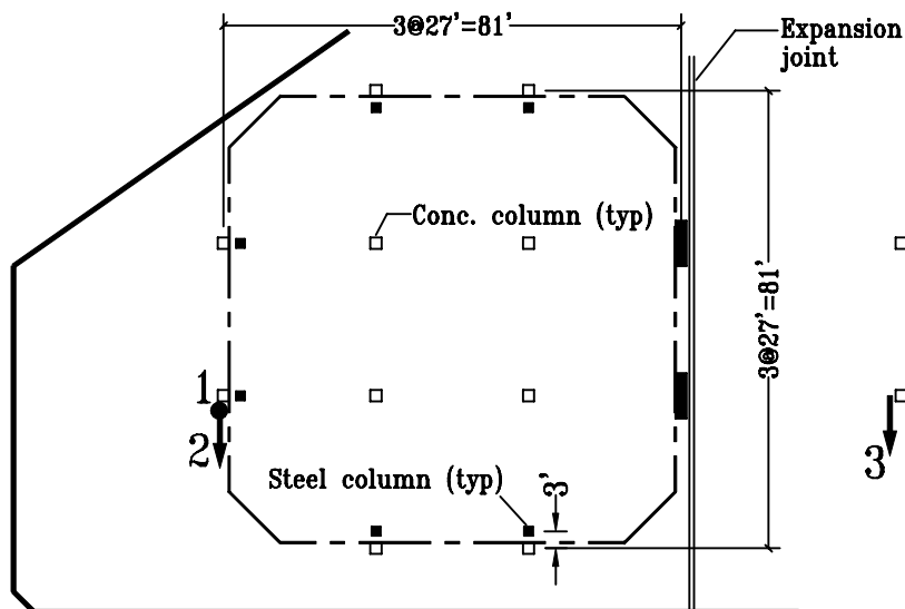
Basement Plan
