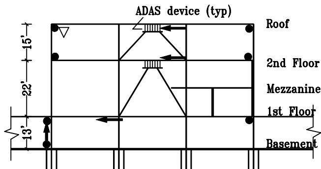
E/W Elevation
