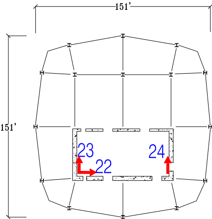
Level 56 Plan
