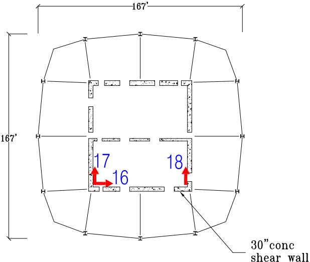
Level 39 Plan
