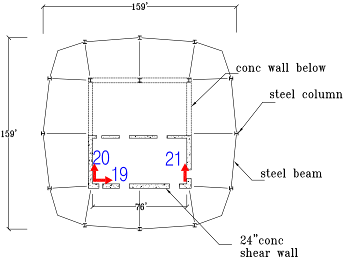
Level 50 Plan
