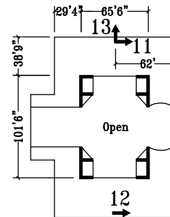
Main Roof Plan
