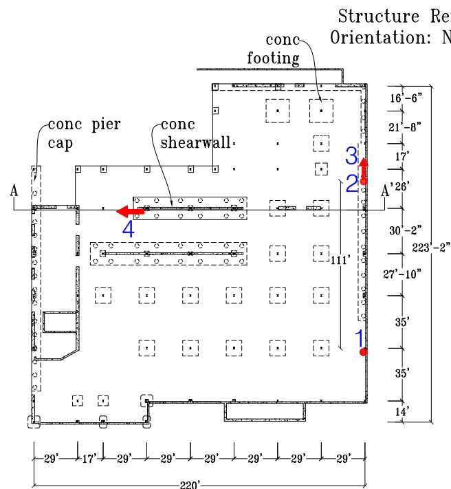
Level 1/Foundation Plan
