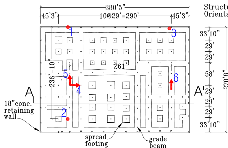
Level P3 (Foundation) Plan
