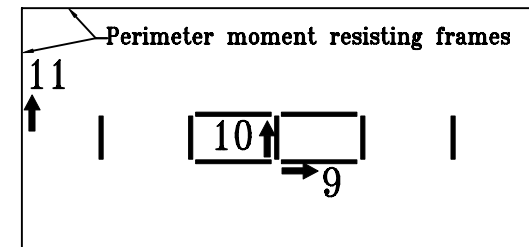
5th Floor Plan
