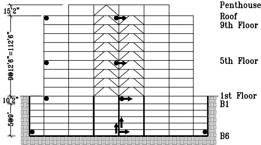
E/W Elevation
