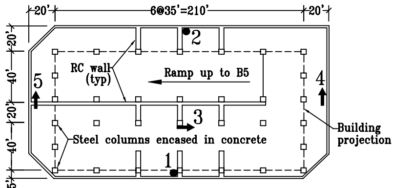
B6 Level Plan
