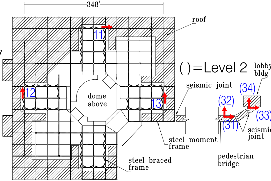
Level 3 Plan
