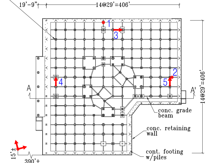
Foundation (Below Isolator) Plan
