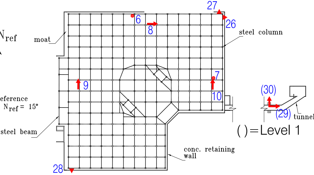
Ground Level (Above Isolator) Plan
