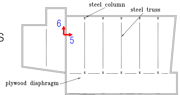
Roof Plan
