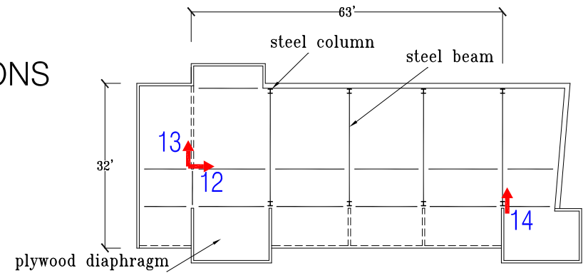
Roof Plan
