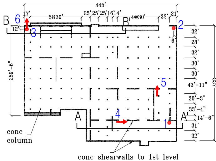
Parking Level Plan
