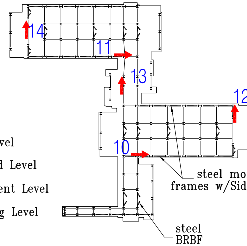
4th Level Plan
