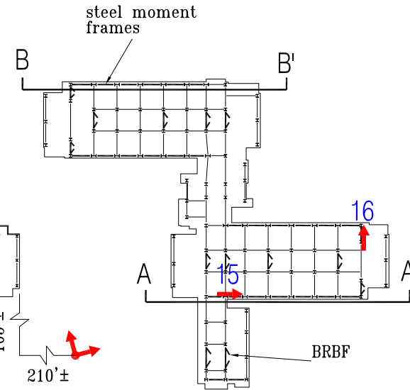
5th Level Plan
