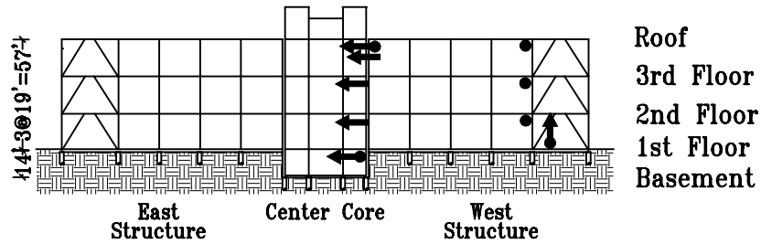
E/W Elevation
