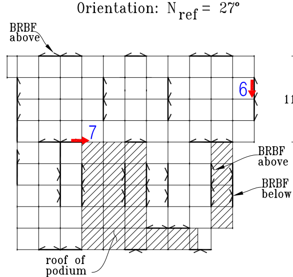
Level 3 Plan
