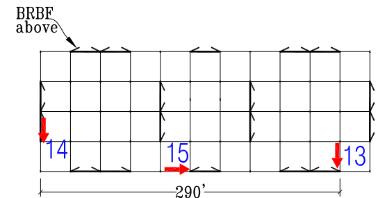
Level 9 Plan
