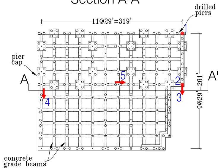
Lower Level (Foundation) Plan
