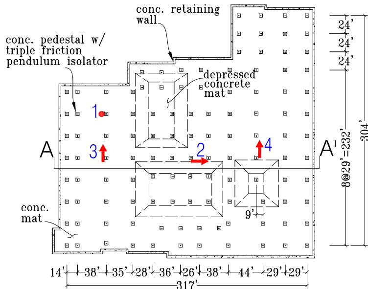
Foundation (Below Isolator) Plan
