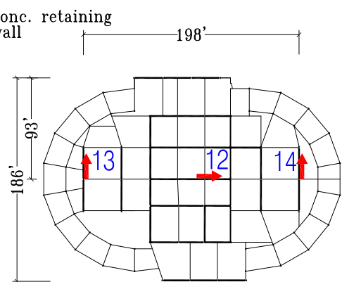
Seventh Floor Plan
