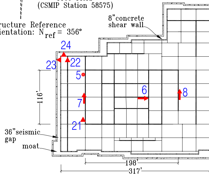
Basement 2 (Above Isolator) Plan
