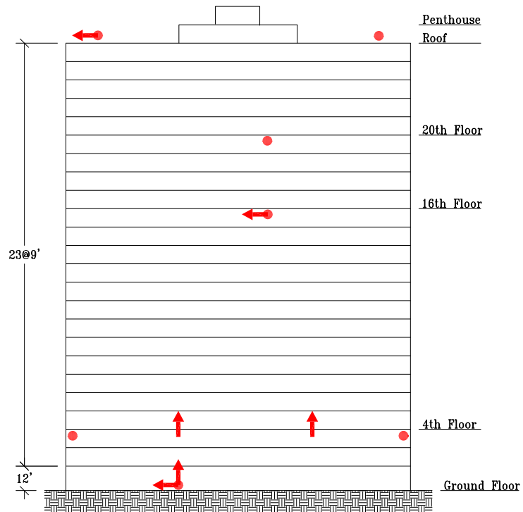
W/E Elevation
