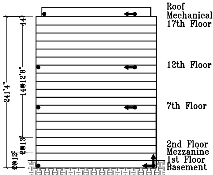
N/S Elevation
