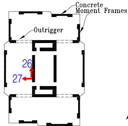
Level 47 Plan
