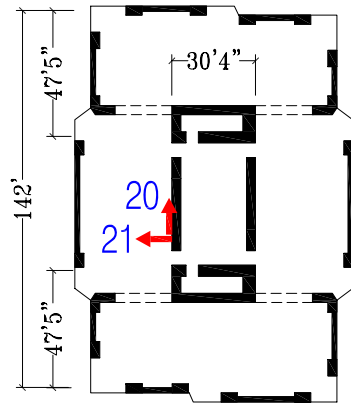
Level 42 Plan
