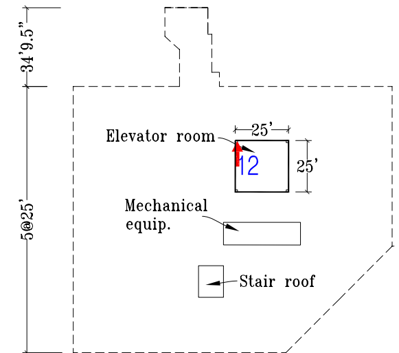
Penthouse Roof Plan
