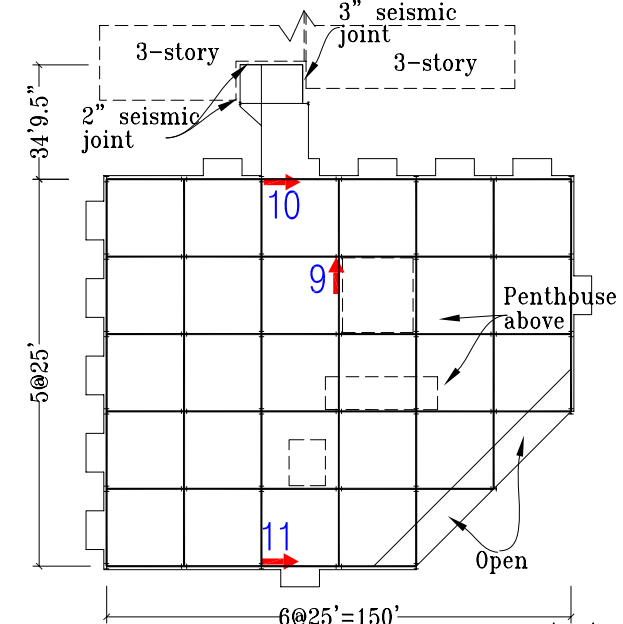
Roof Plan
