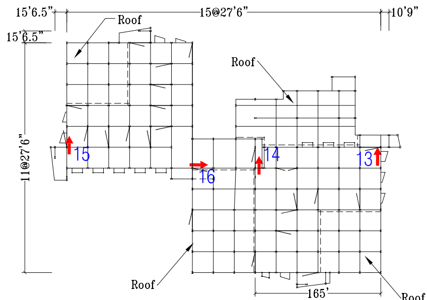
Level 3 Plan
