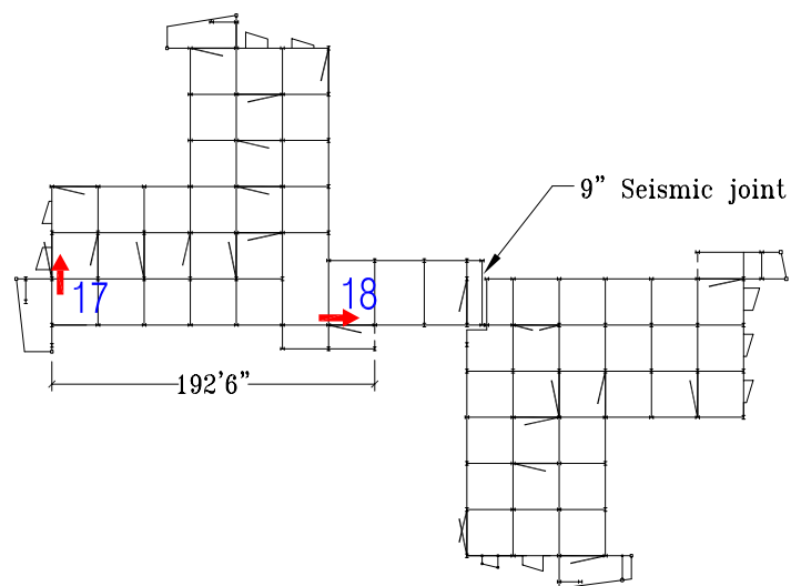
Level 5 Plan
