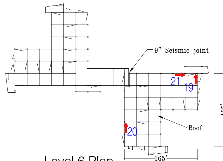
Level 6 Plan
