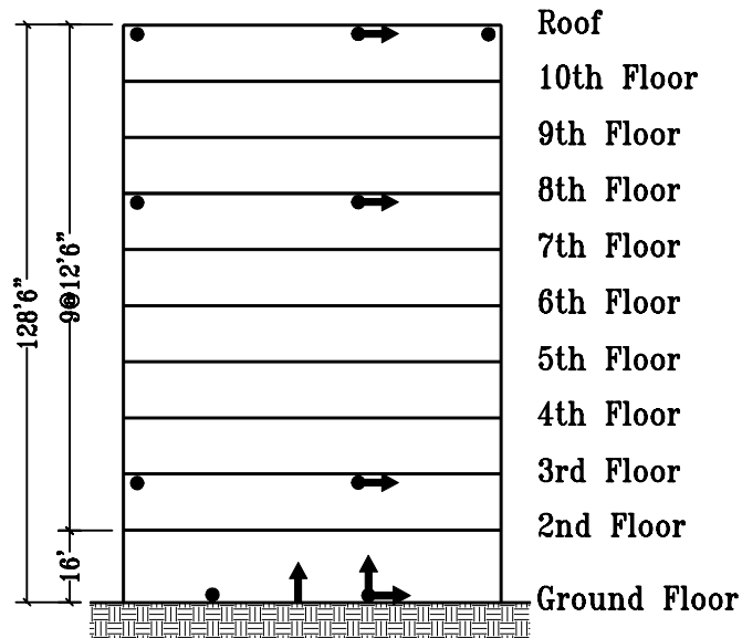
N/S Elevation
