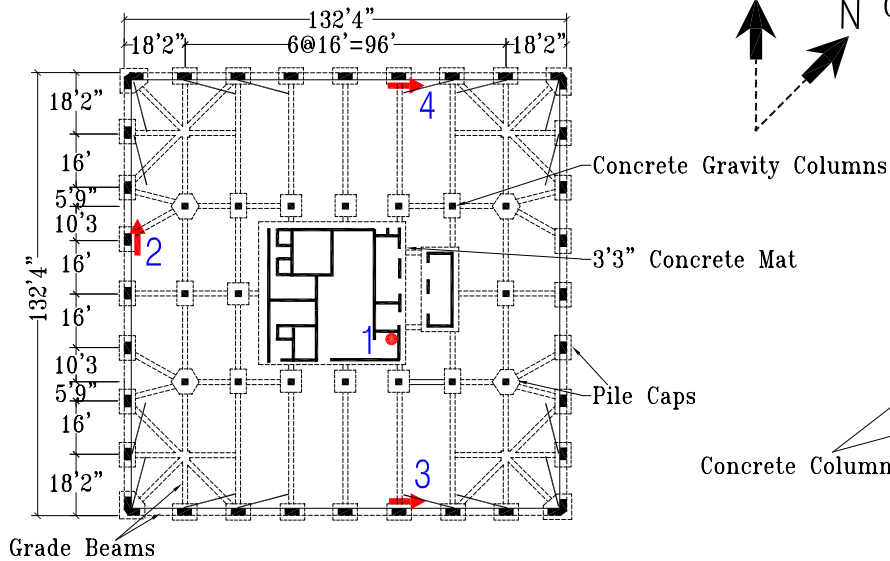
Ground Floor/Foundation Plan
