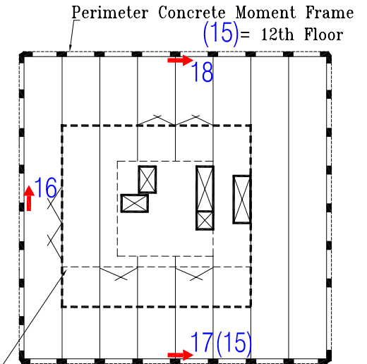
Roof plan
