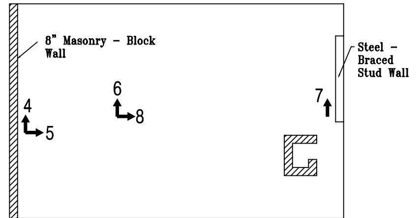
Roof Plan
