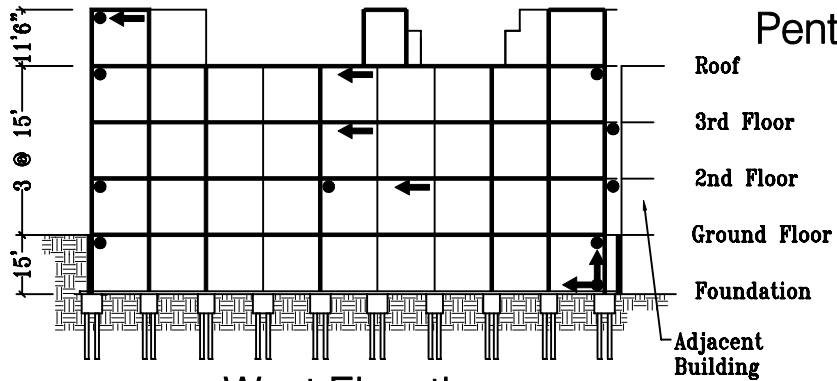
West Elevation
