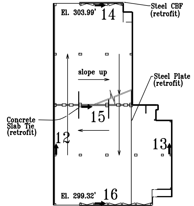
Roof Plan
