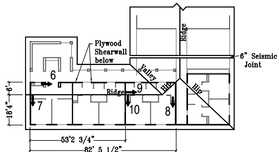
Roof Plan
