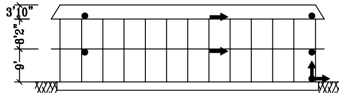
Elevation Wing B
