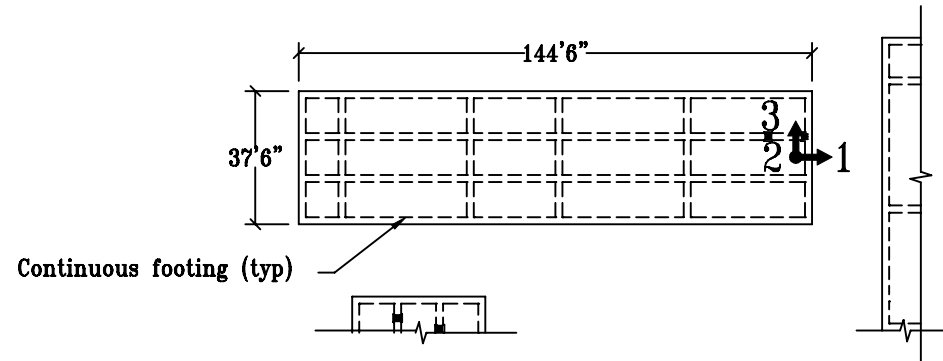
1st Floor Plan Wing B
