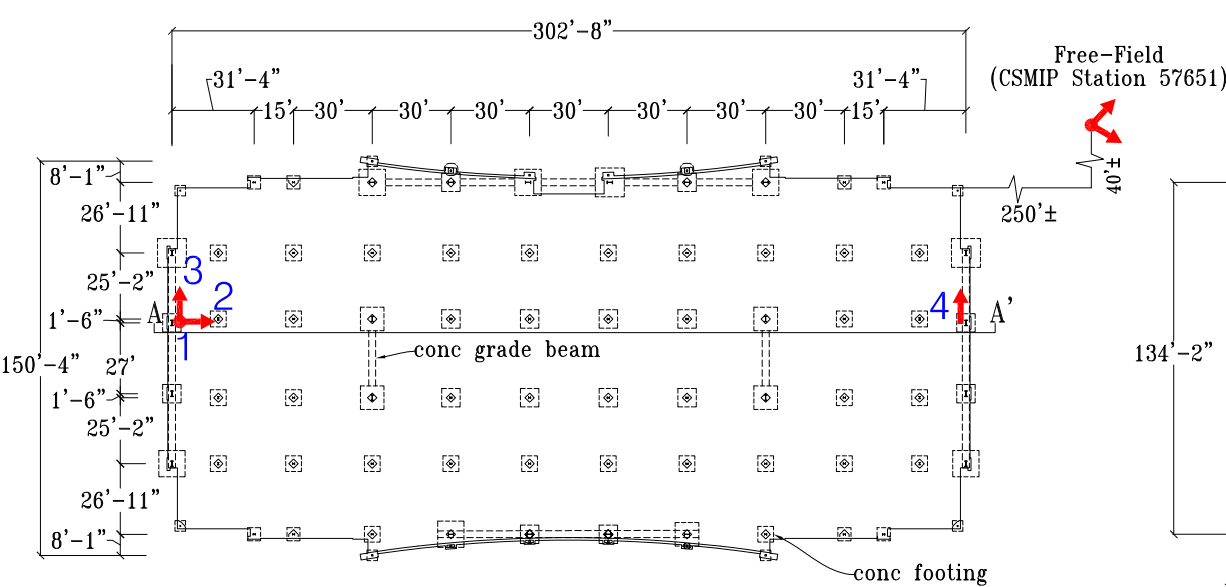
Foundation/First Floor Plan
