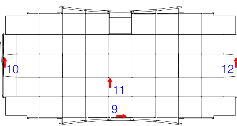
Roof Plan
