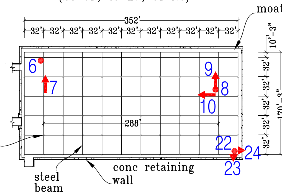
Ground Floor (Above Isolator) Plan
