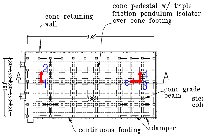
Foundation (Below Isolator) Plan
