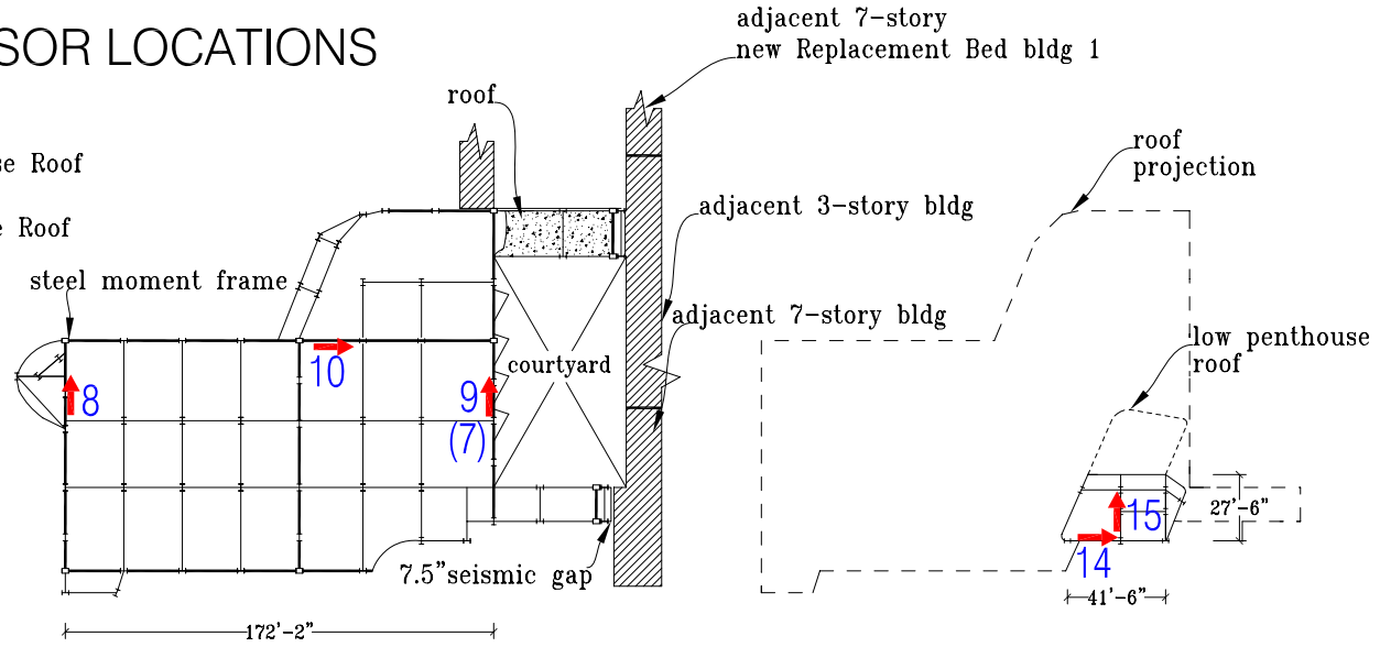
Fourth Floor Plan ( ) = 3rd Floor
