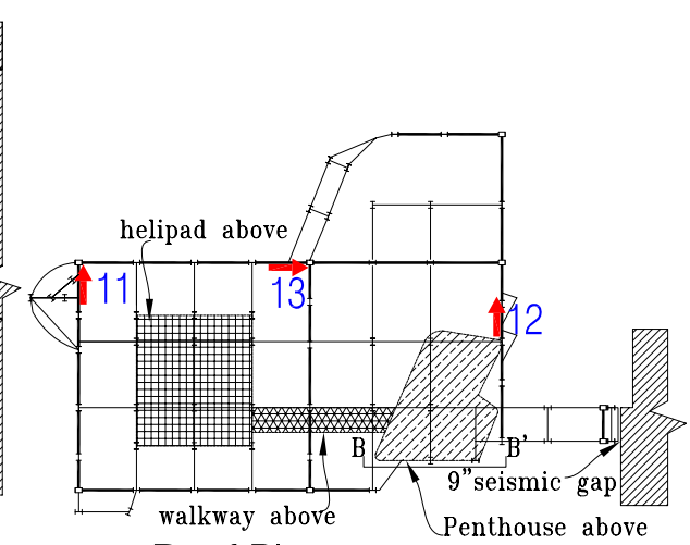
Roof Plan
