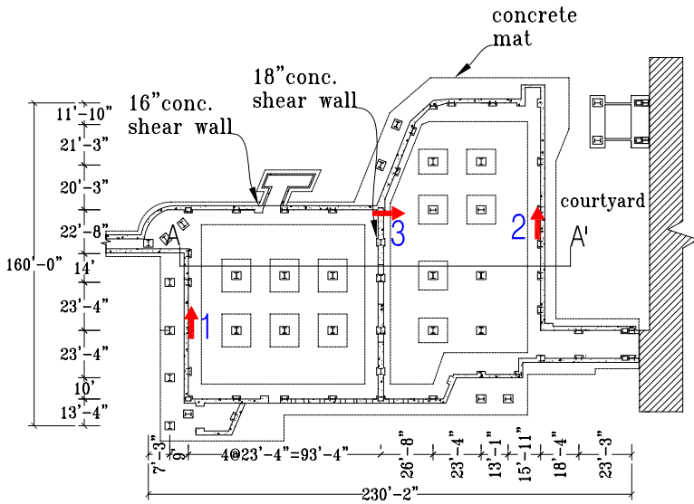
Basement Plan
