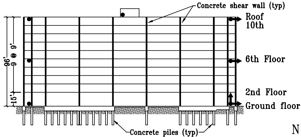
N/S Section
