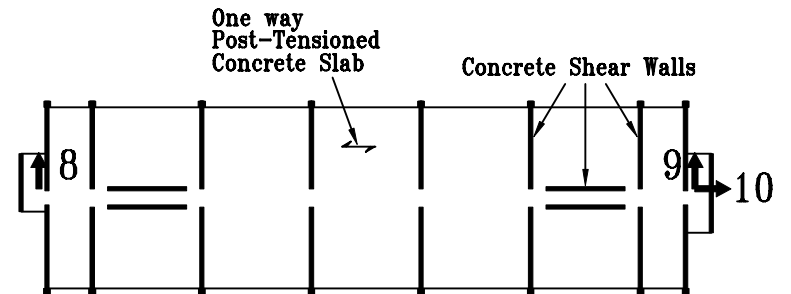
6th Floor Plan
