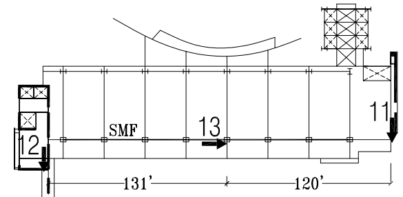
Level 9 Plan
