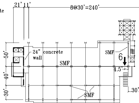
Level 2 Plan
