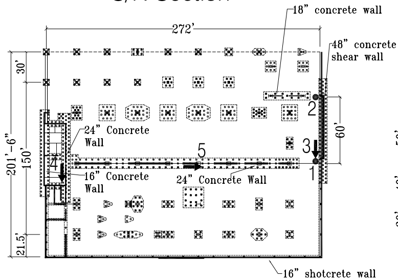
Level P1 Plan
