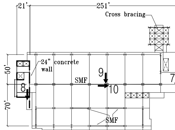
Level 4 Plan
