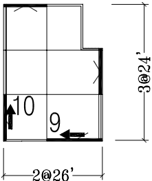
Penthouse Roof Plan
