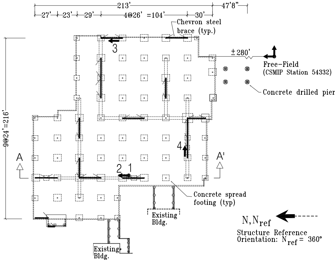
Ground Floor/Foundation Plan
