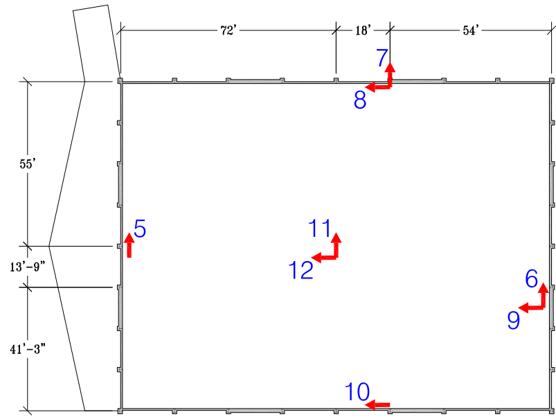
Roof Plan
