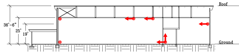
W/E Elevation
