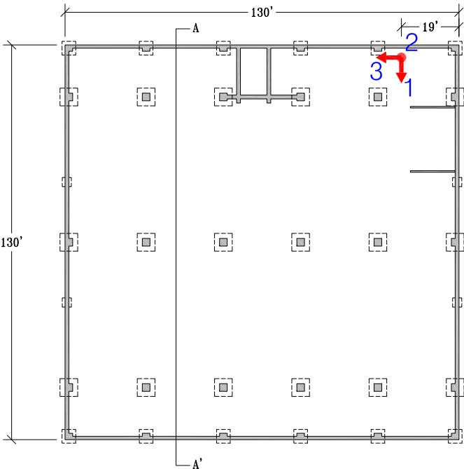
Foundation Plan
