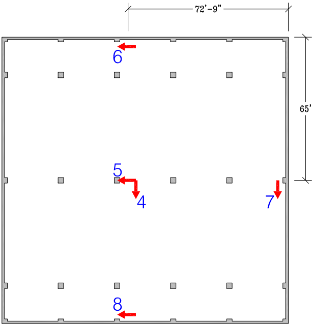
Roof Plan
