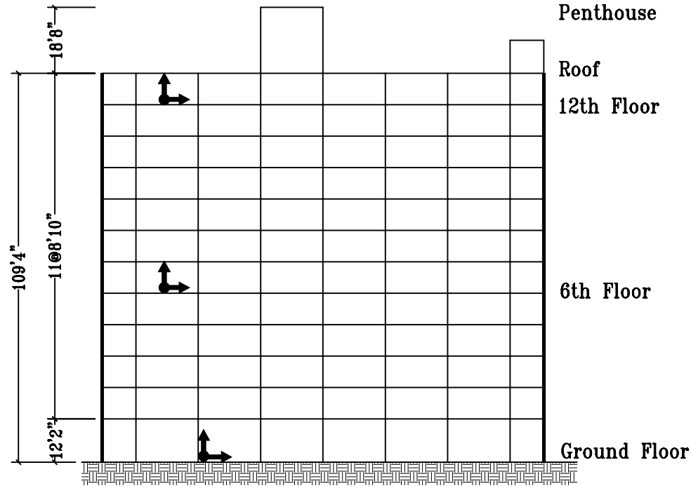
W/E Elevation
