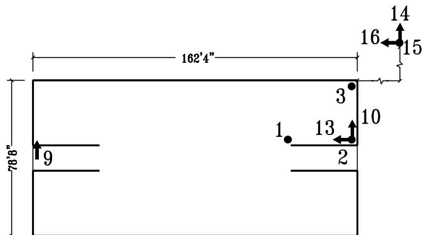
Foundation Plan
