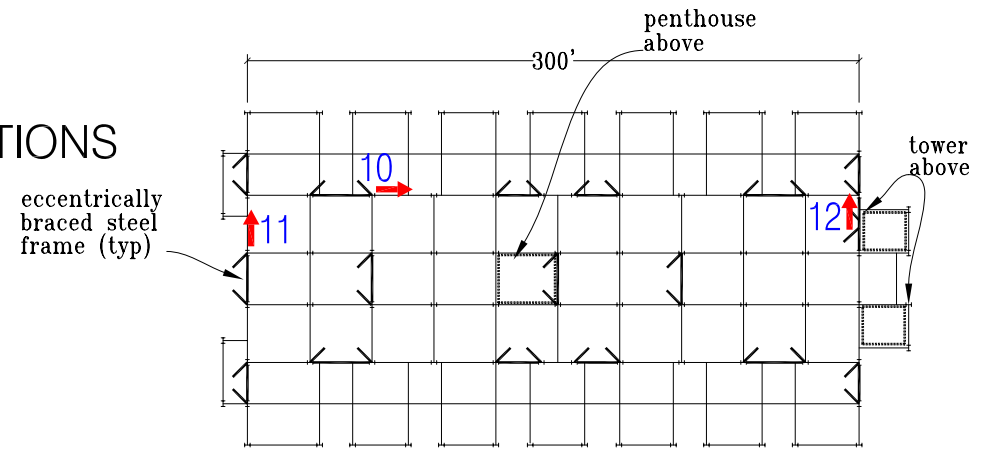
Roof Plan
