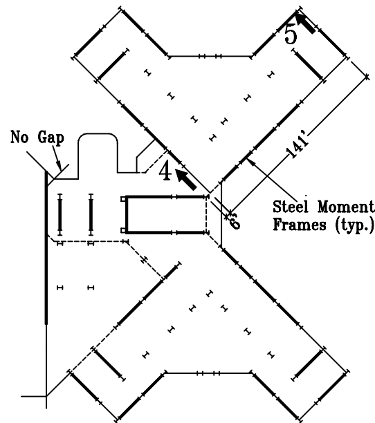
Mall Level Plan
