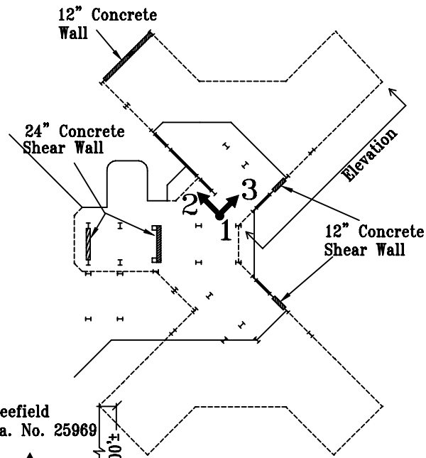
Garden Level Plan
