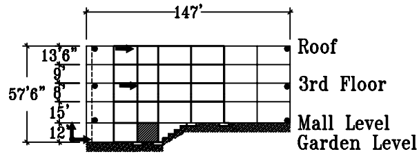
Elevation (NE Wing Only)
