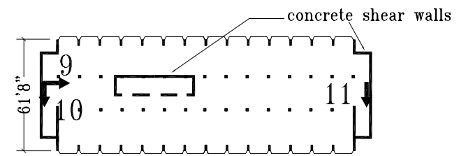
4th Floor Plan
