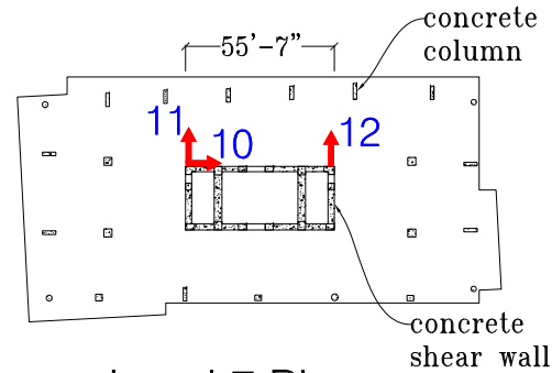
Level 7 Plan
