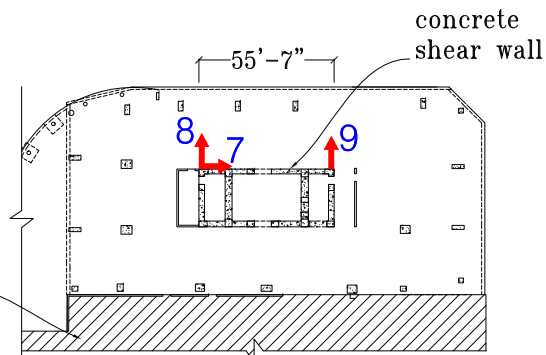
Level 1 Plan
