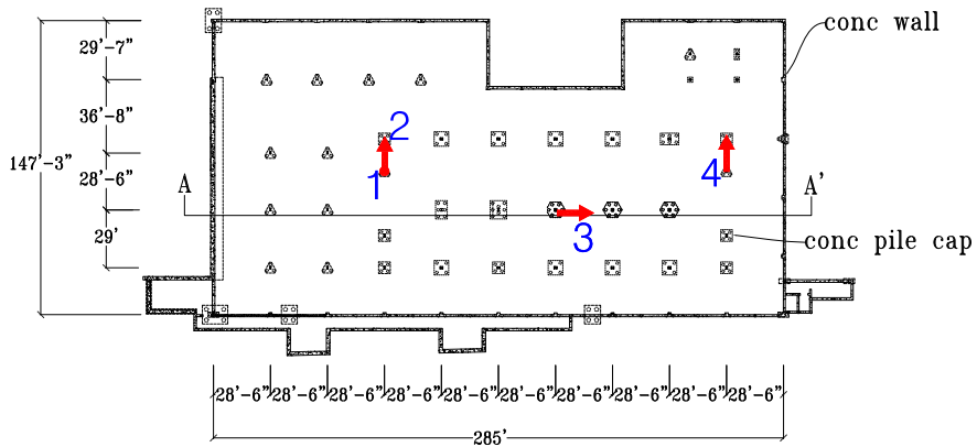
Sub-basement/Foundation Plan
