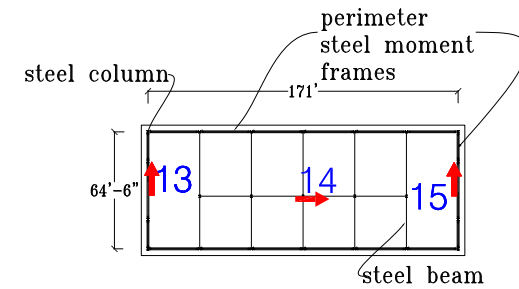
Roof Plan
