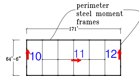
Seventh Floor Plan
