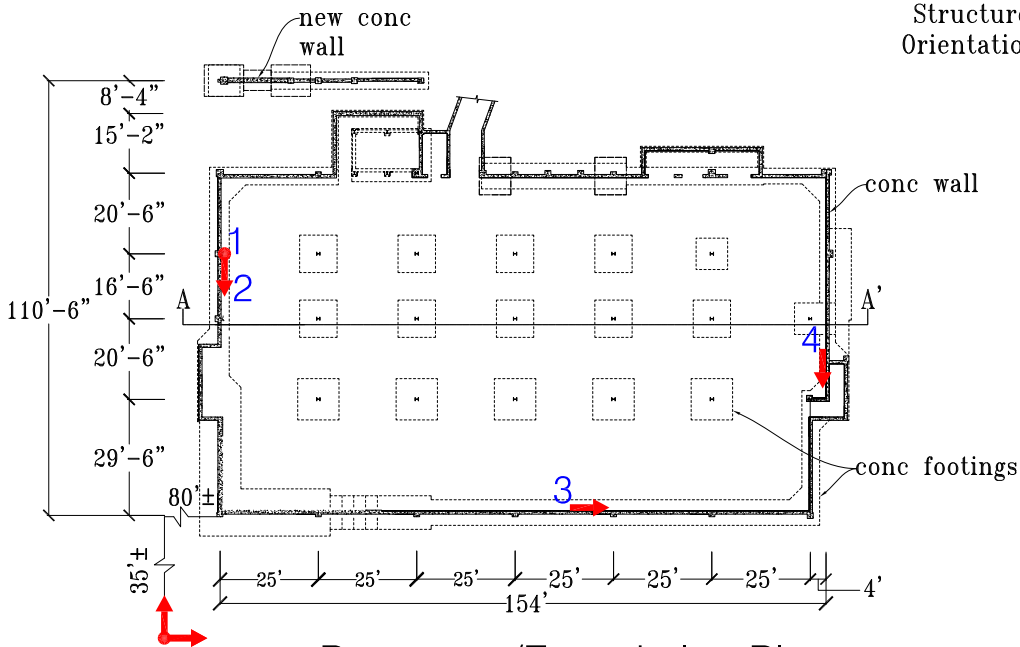
Basement/Foundation Plan
