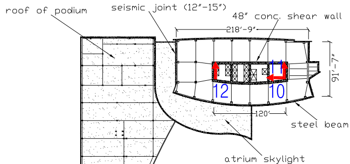
11th Floor Plan
