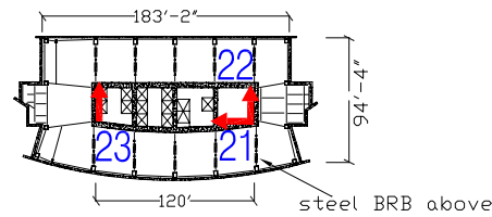
53rd Floor Plan
