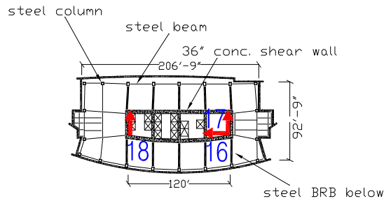
31st Floor Plan
