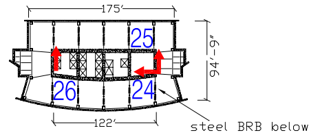
59th Floor Plan
