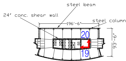
41st Floor Plan
