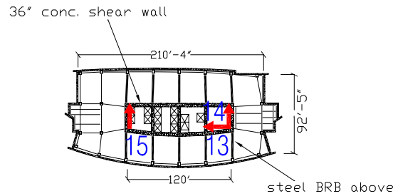
28th Floor Plan
