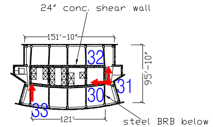
73rd Floor Plan
