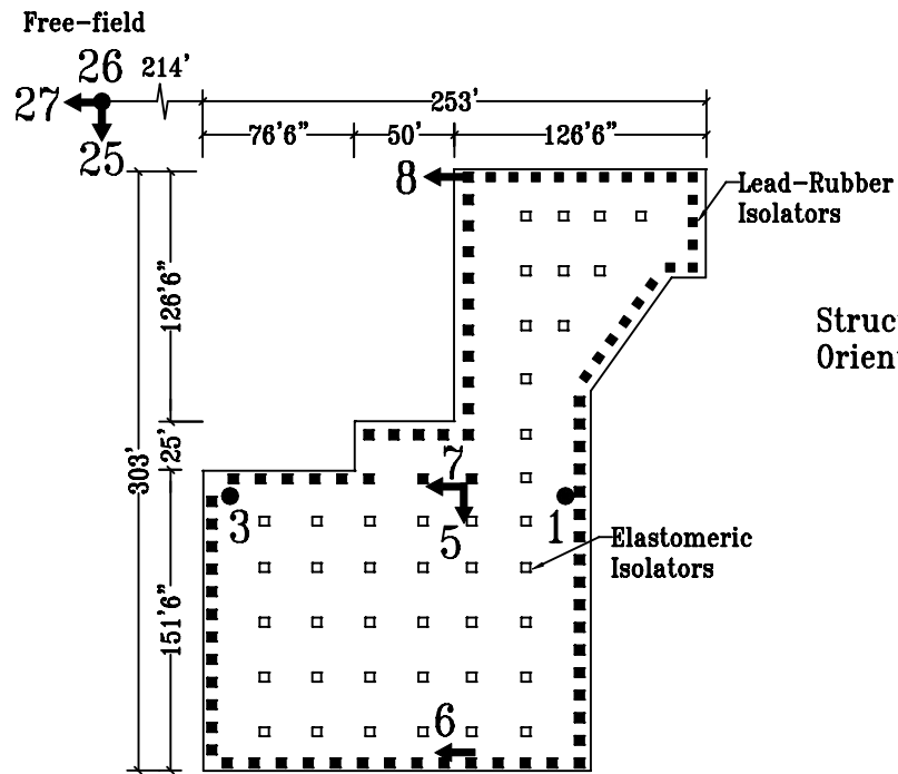
Foundation Level
