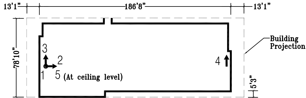
Basement Plan
