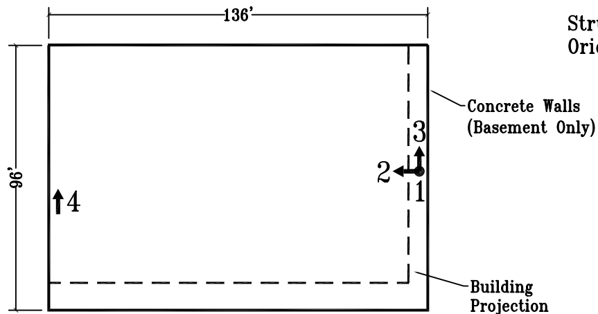
Basement Plan
